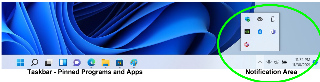
Figure 1 - 15 - Taskbar
